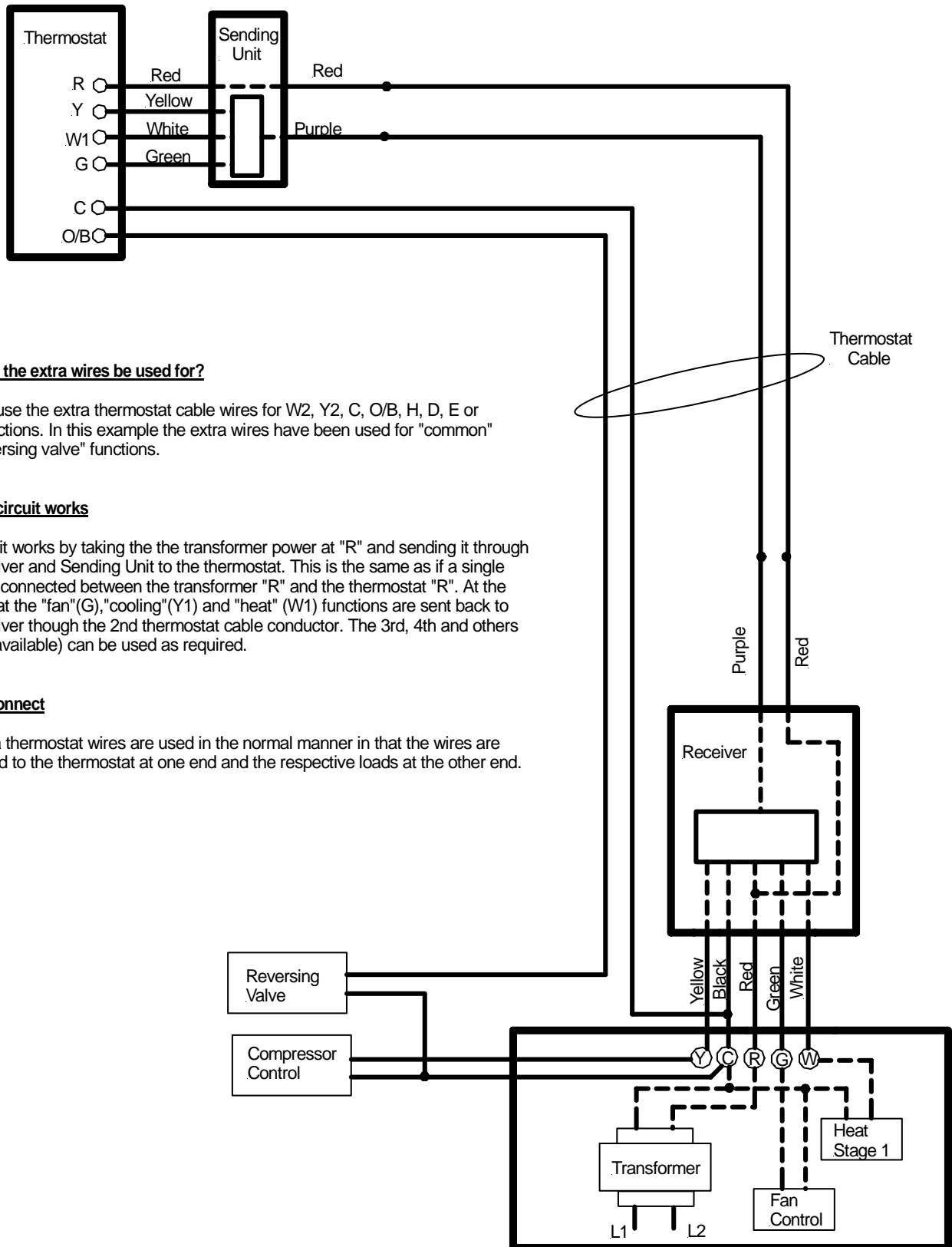
Furnace Wiring
